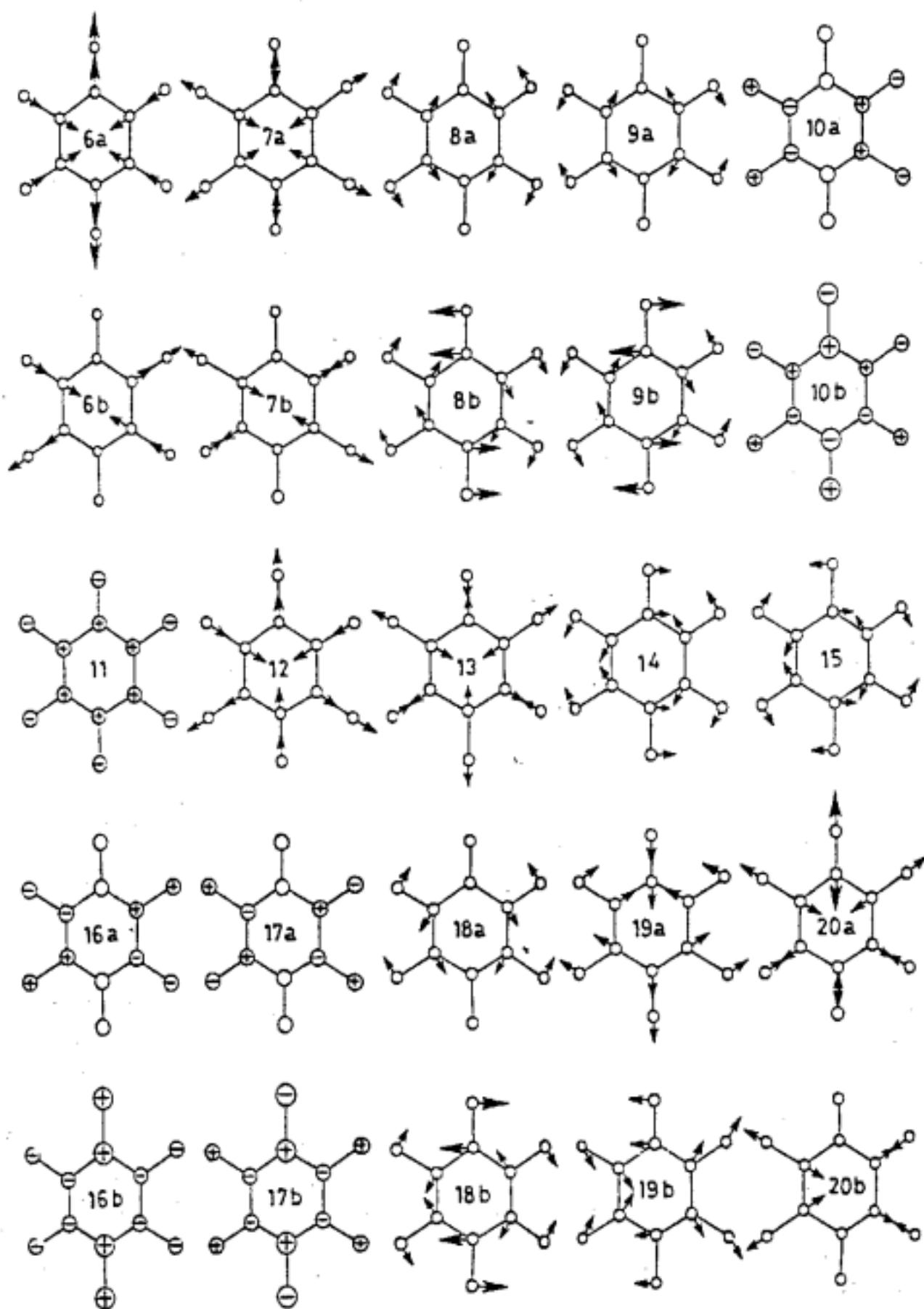
Fig. 1. Normal vibrations of benzene
